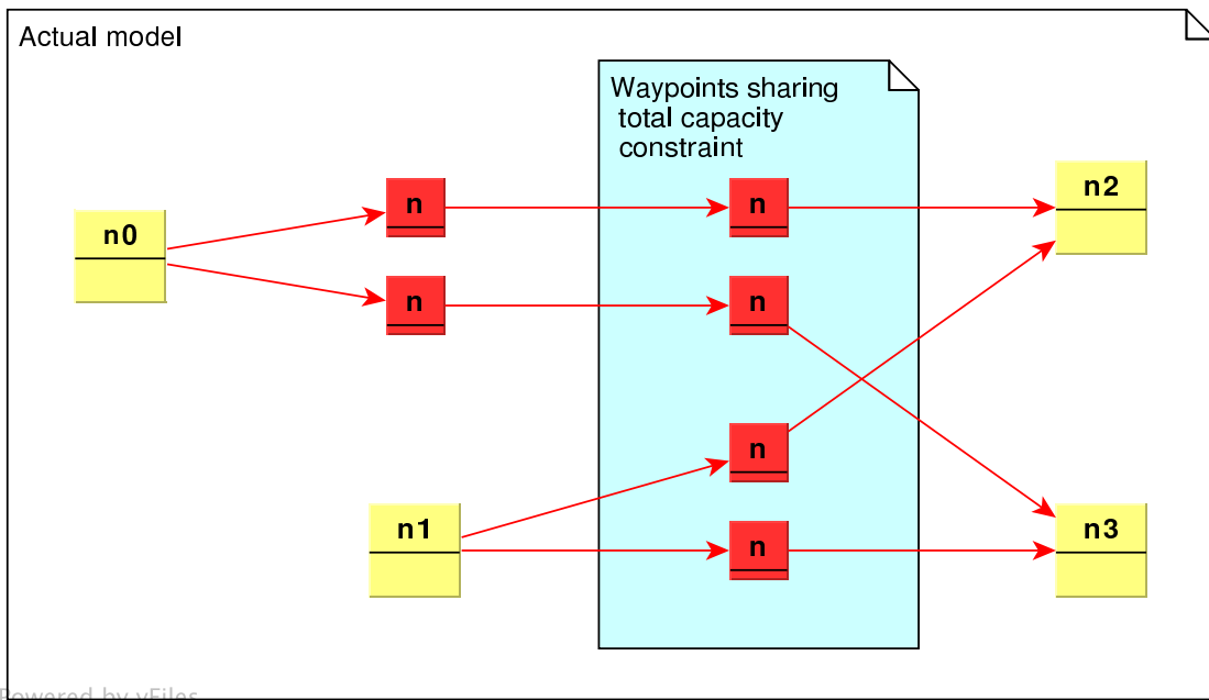
Figure 6.1: Constraint Pooling
