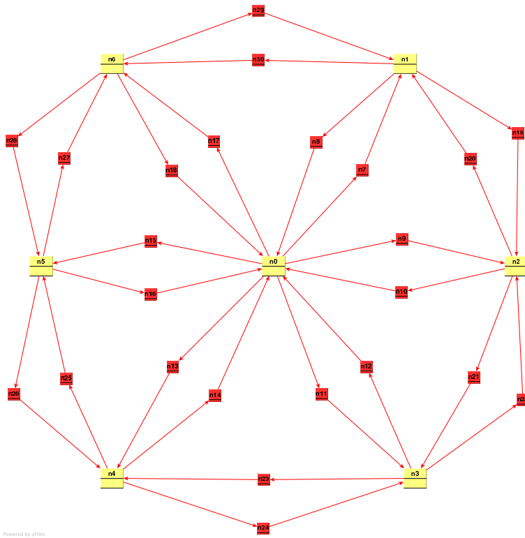
Figure 5.6: 2D Hexagonal Cluster
